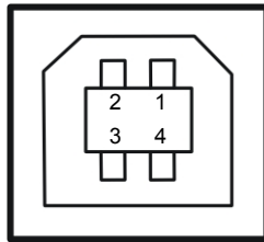
Figure 5-2 USB interface
