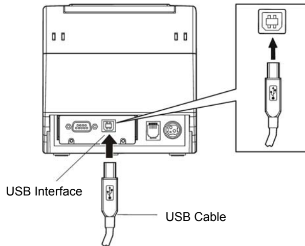
Figure 2-4 Connecting the USB cable
