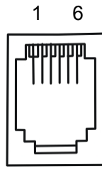
Figure 5-7 Cash drawer connector
