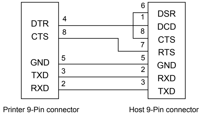
Figure 5-4 Connecting with 9-Pin PC
