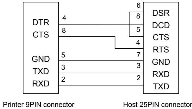
Figure 5-5 Connecting with 25-Pin PC
