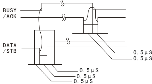
Figure 5-1 Timing signal in parallel interface
