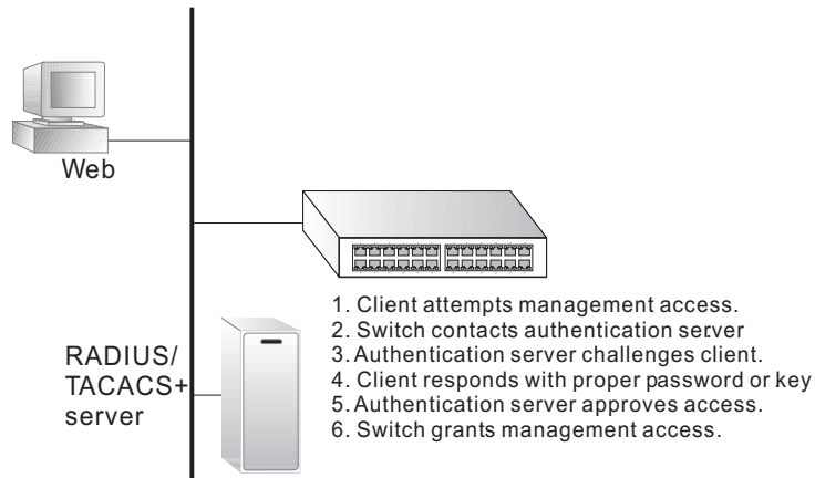
Figure 16: Authentication Server Operation
