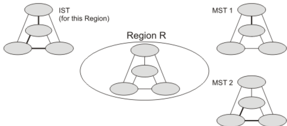
Figure 44: MSTP Region, Internal Spanning Tree, Multiple Spanning Tree
