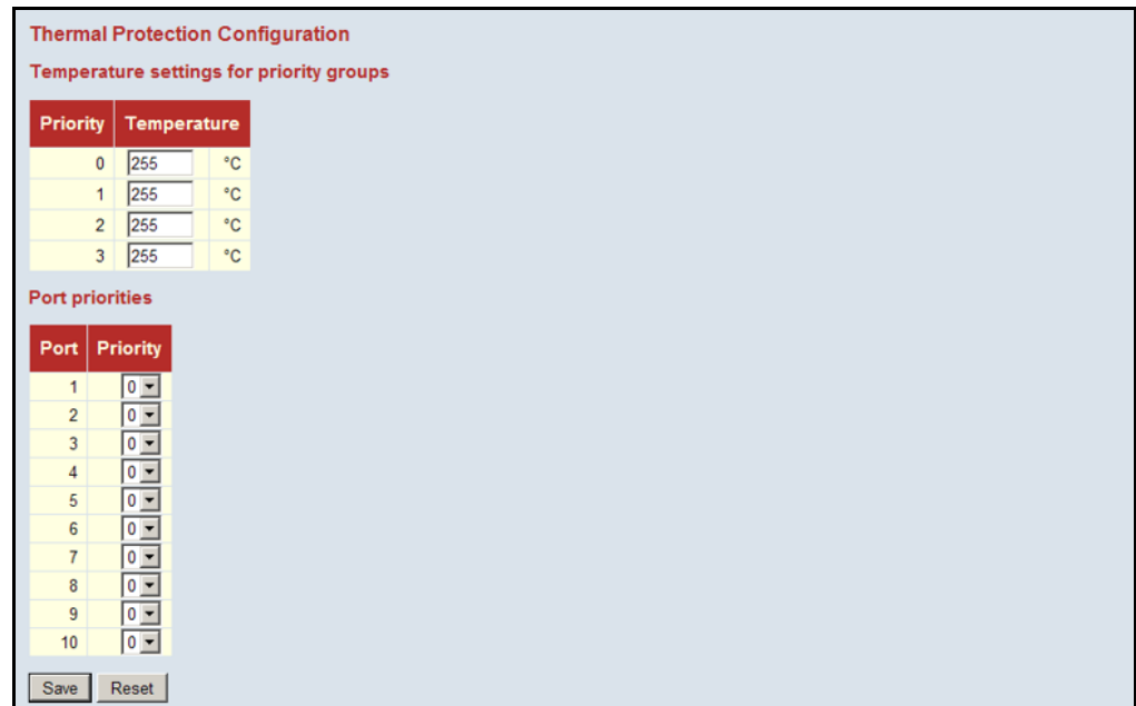
Figure 11: Configuring Thermal Protection
