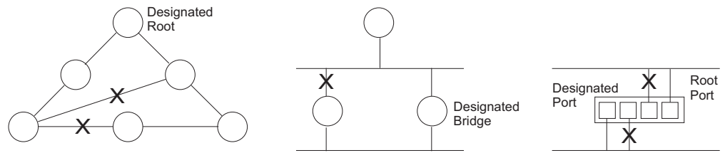
Figure 43: STP Root Ports and Designated Ports
