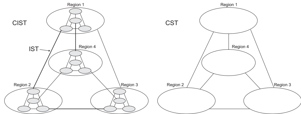
Figure 45: Spanning Tree – Common Internal, Common, Internal
