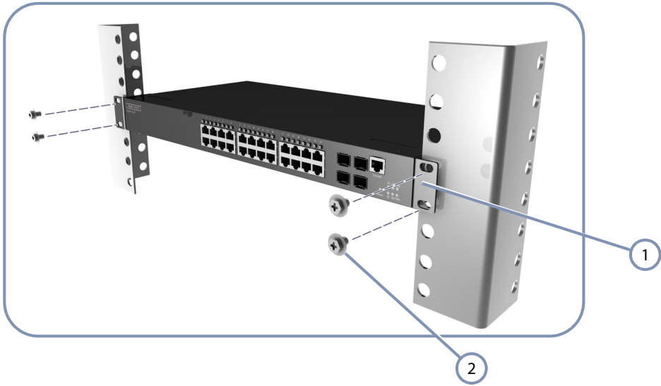
Figure 3: Installing the Switch in a Rack
