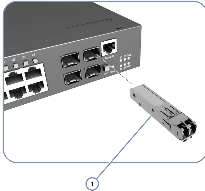
Figure 17: Inserting an SFP Transceiver into a Slot
