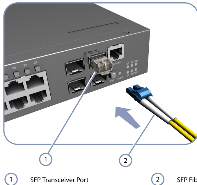
Figure 20: Making a Connection to an SFP Port
