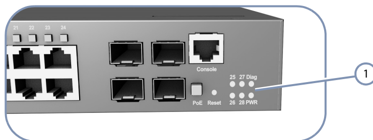
1 System Status LEDs
