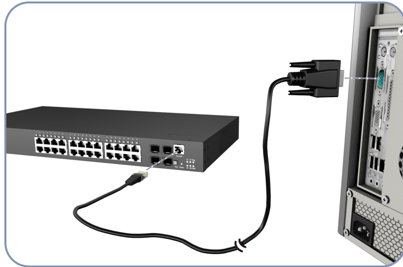
Figure 23: Console Port Connection
