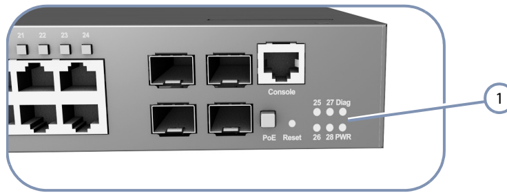
Figure 5: System LEDs
