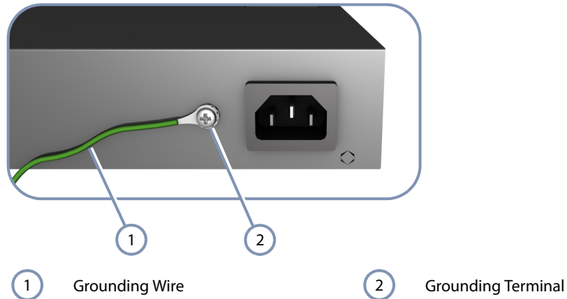
Figure 14: Grounding Terminal
