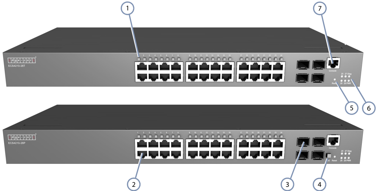
Figure 1: Front Panel ECS4210-28T and ECS4210-28P
