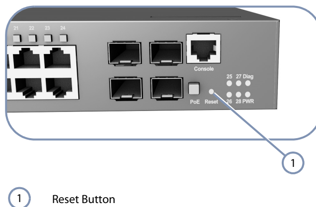
Figure 24: Reset Button
