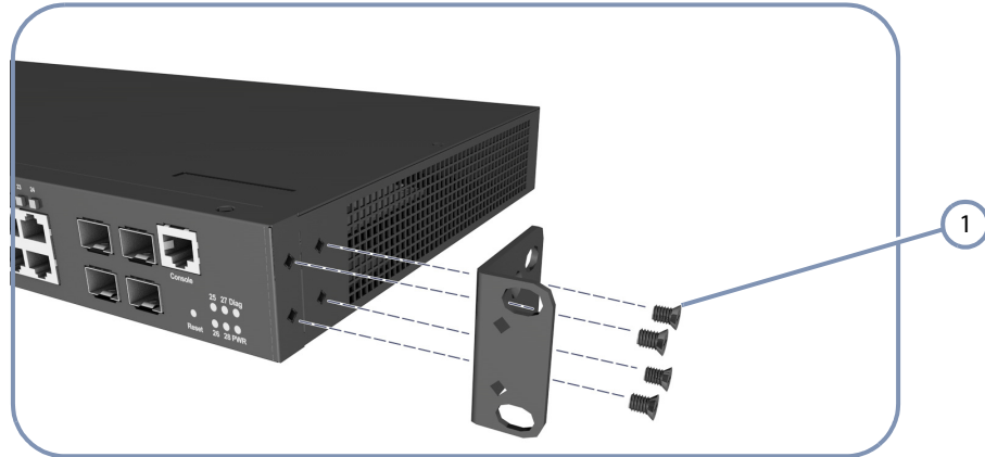
Figure 8: Attaching the Brackets
