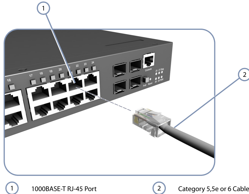
Figure 19: Making Twisted-Pair Connections
