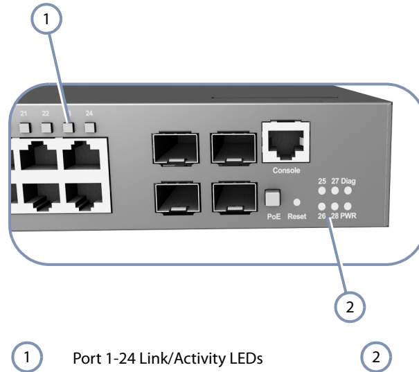
Figure 16: Port Status LEDs
